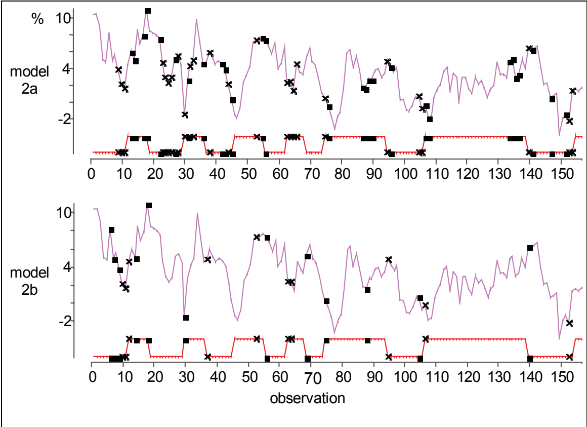
Figure 4: Support vectors and crossvalidated errors (GNP, models 2a and 2b)
