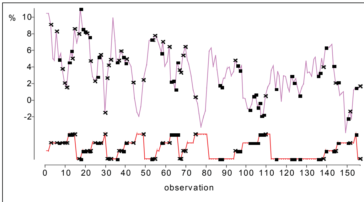
Figure 6: Support vectors and crossvalidated errors (GNP, model 1a)
