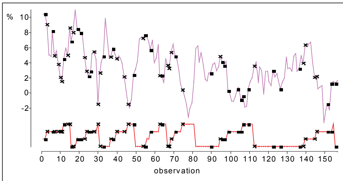
Figure 7: Support vectors and crossvalidated errors (GNP, model 1b)
