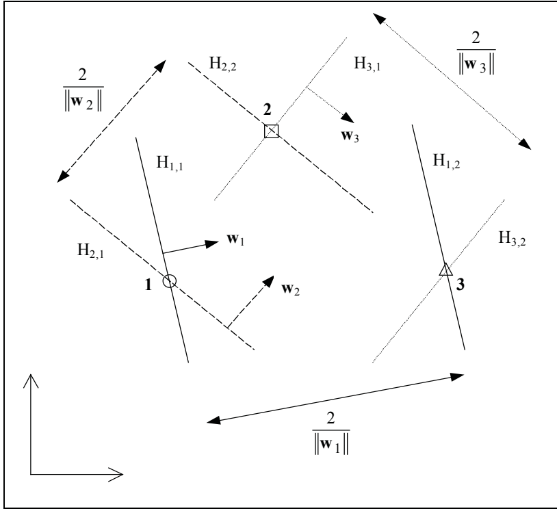
Figure 2: Multi-class separation
