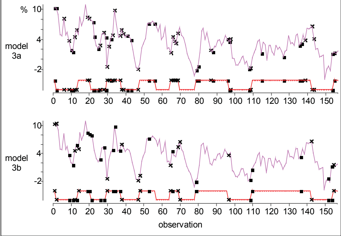
Figure 5: Support vectors and crossvalidated errors (GNP, models 3a and 3b)
