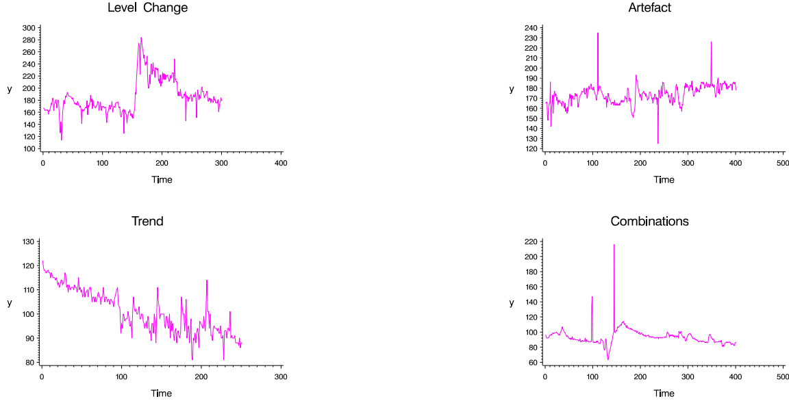
Figure 1: Patterns of change in univariate physiologic time series. Combinations of several patterns, which usually occur in practice, may cause problems for any identification rule
