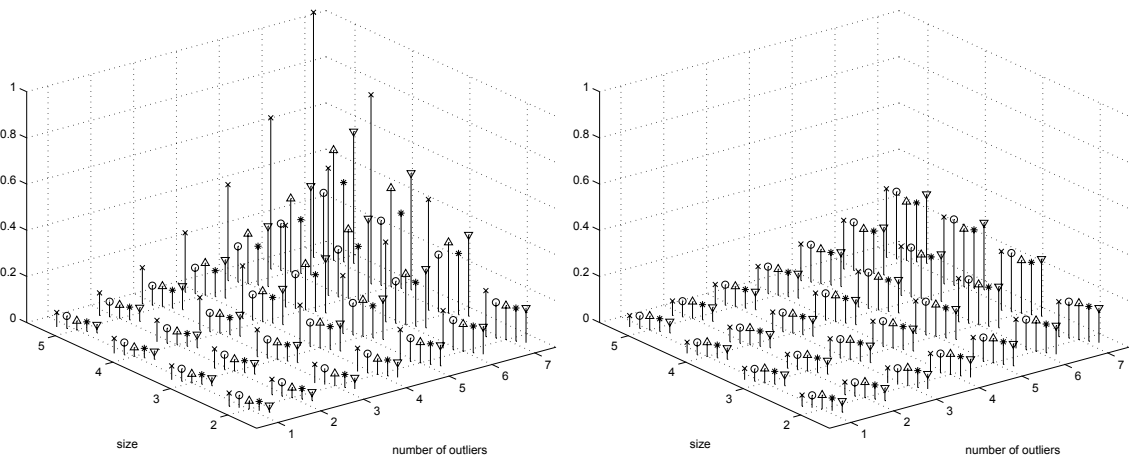
Figure 1: Moderate number of small to medium-sized outliers: Simulated MSE for MAS \times , MAD \circ , SN \triangle , TMM * , QN \nabla (left), and LSH \times , LTS \circ , SMAD \triangle , TS * , IQR \nabla (right).
