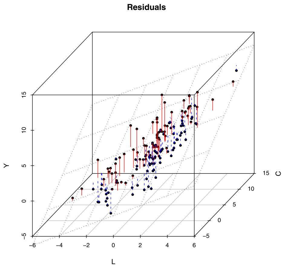
Figure 8: Residuals (cf. Figure 7)
