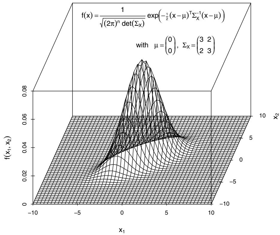
Figure 5: Density of a bivariate normal distribution
