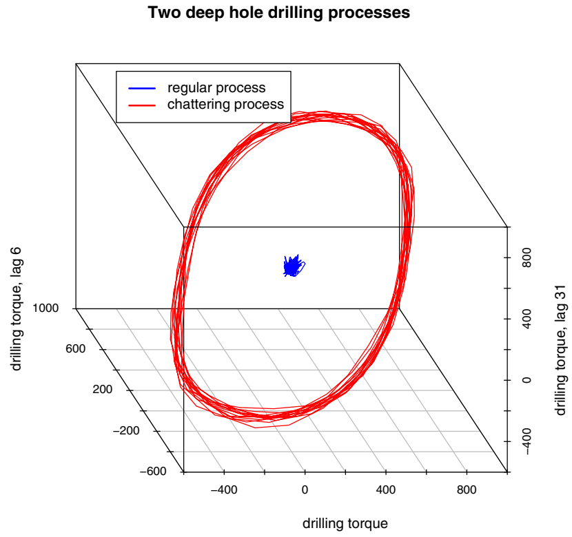
Figure 9: Phase spaces of the drilling torques of two deep hole drilling processes
