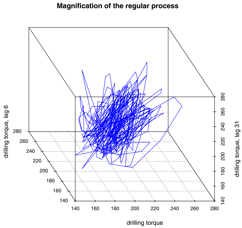
Figure 10: Magnification of the regular process (Figure 9)
