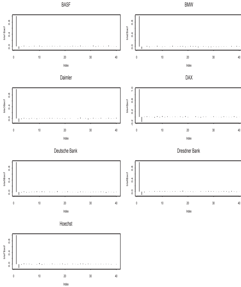
Figure 2: Autocorrelations of the residuals of absolute daily returns of seven German stocks
