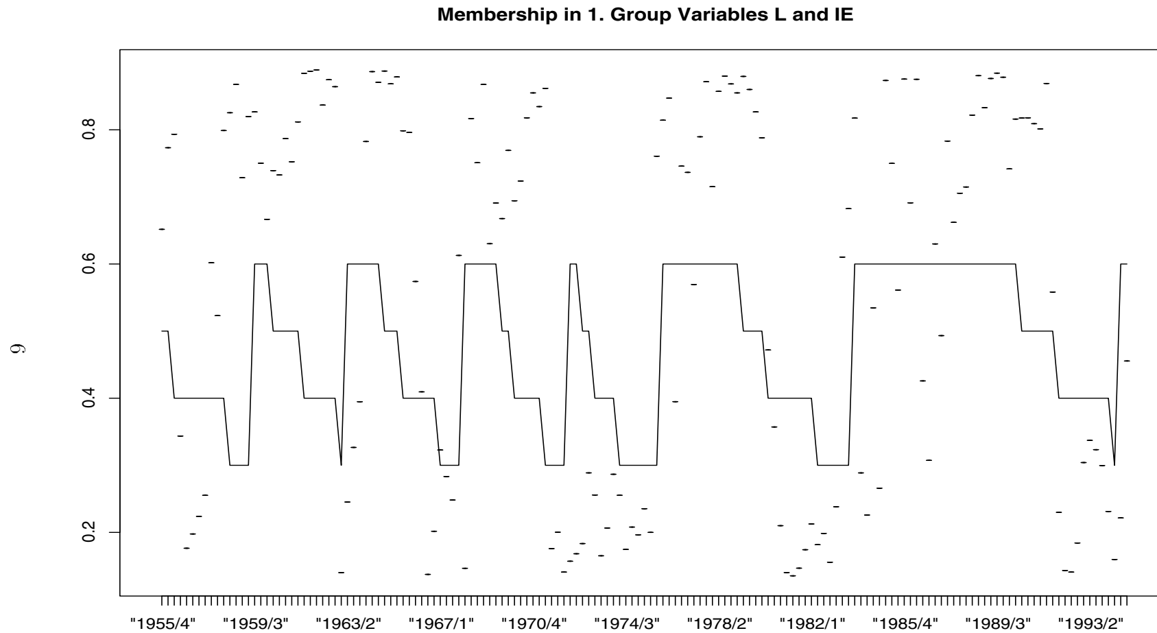
Figure 3: Memberships in 1. Group using raw data cp. to 4-phase-scheme
