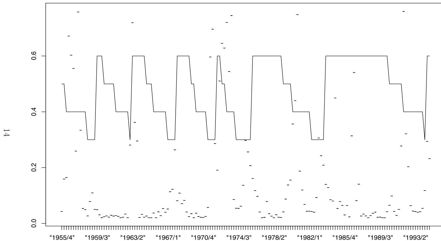
Figure 10: Membership in Group 2, using 3 groups and normalization
