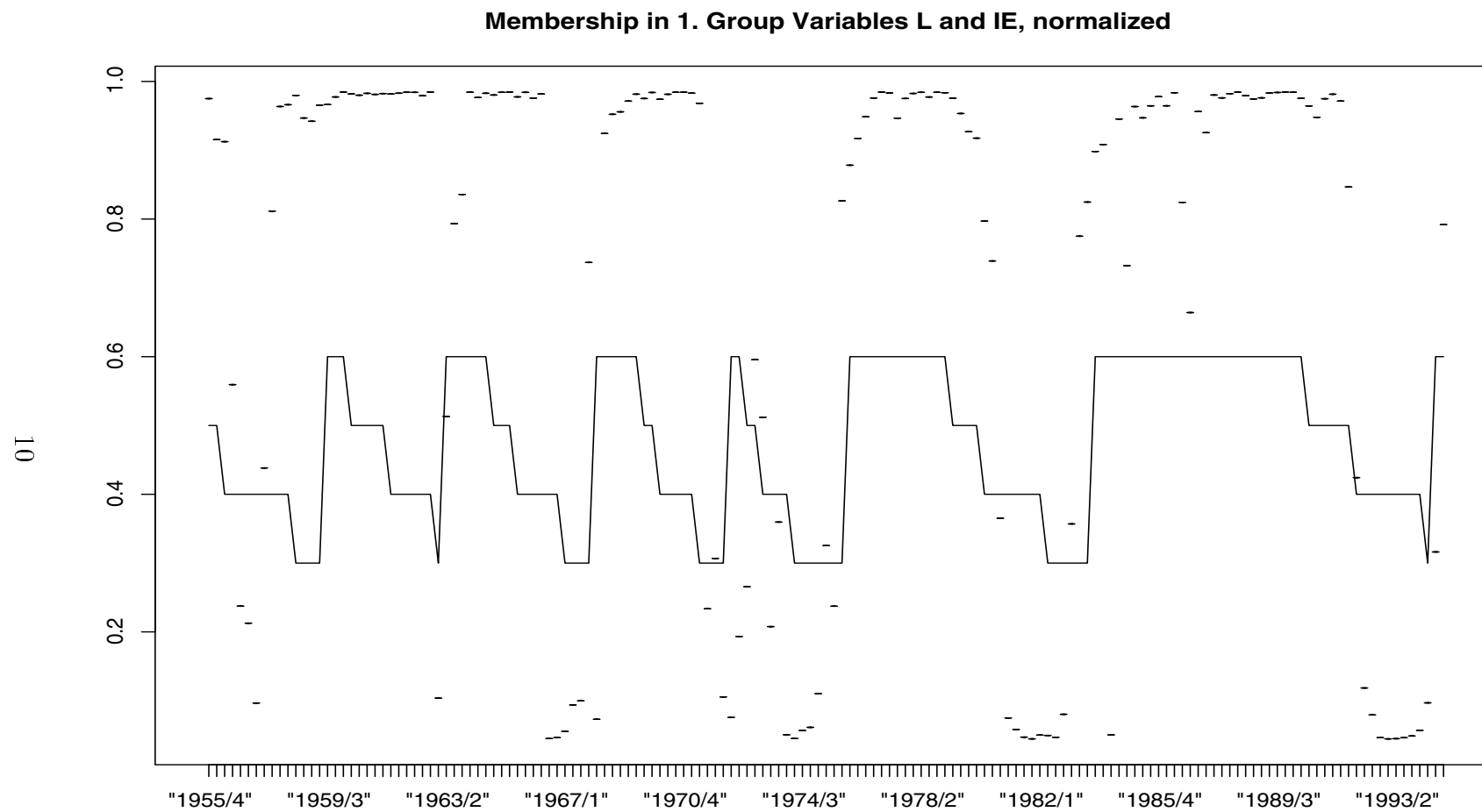
Figure 7: Memberships in group 1 for normalized data and Variables L and IE
