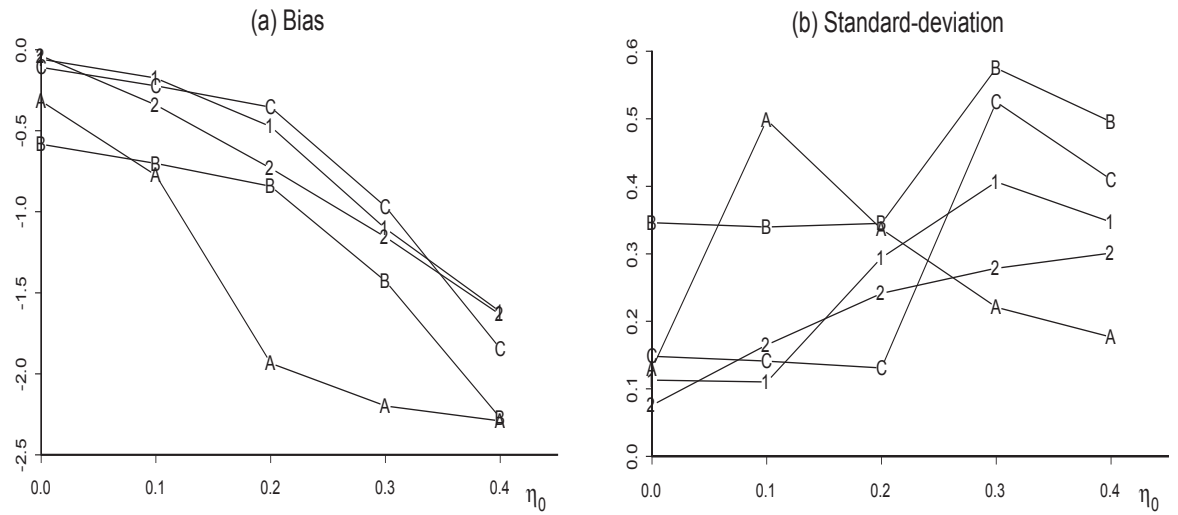
Figure 9: Bias and standard-deviation of some L- and MS-estimators with N = 50 , \theta = 2 , b = 16 , \eta_1 = 0.2 ; MS-estimators based on – 1 – : MAD , – 2 – : RCS ; L-estimators with – A – : r = 5 , s = 0 , – B – : r = 13 , s = 5 , – C – : r = 13 , s = 13 .
