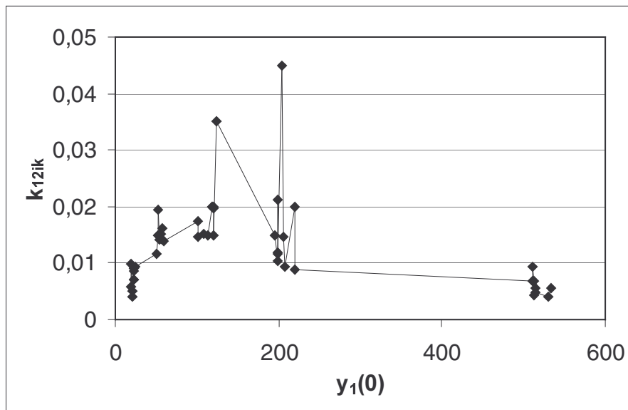
Figure 4. Comparison of maximum likelihood estimates of k_{12ik} and estimated maximum concentration in the first compartment.
