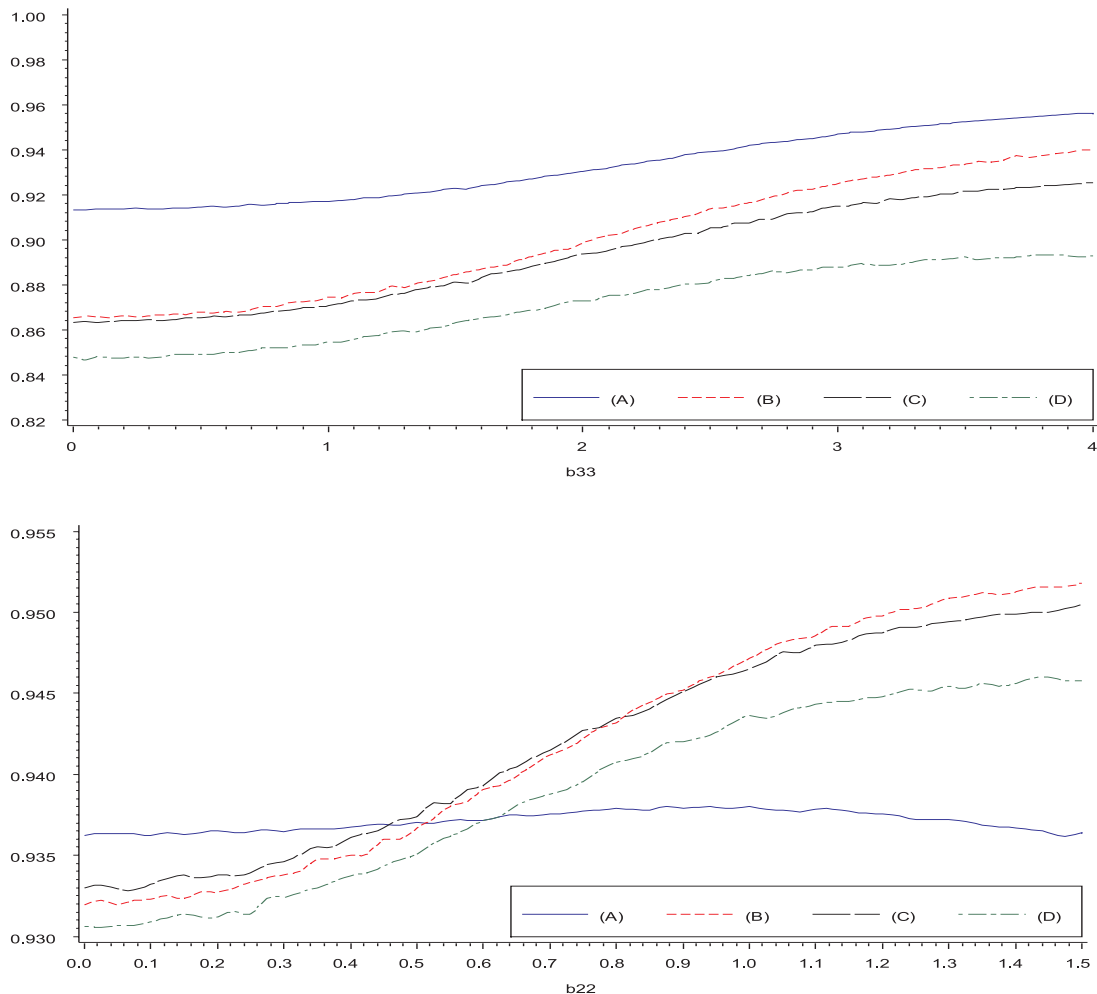
Figure 3.2: Simulated D -efficiencies of the sequential designs (3.3) proposed by Biswas and Chaudhuri (2002) in the identified polynomial regression model (3.1). Figure 3.2a (upper panel): cubic model is "correct"; Figure 3.2b (lower panel): quadratic model is "correct".
