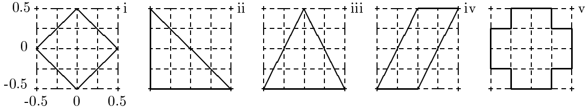
Figure 1. Examples of templates R_0 \subset (-1/2, 1/2]^2 are outlined by solid lines. Cross-shaped sampling regions R_n described in Table 2 are based on R_0 in (v).
