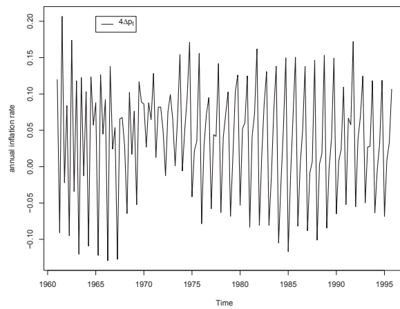
Figure 4: Time series used
