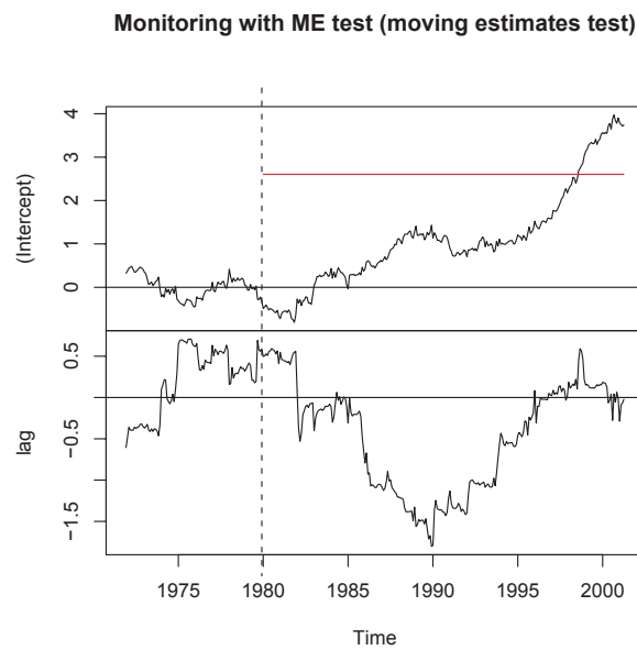
Figure 12: 2-dimensional moving estimates process
