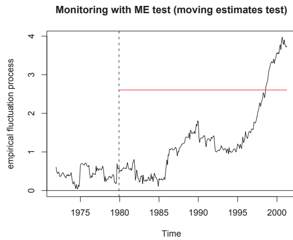
Figure 11: Moving estimates process
