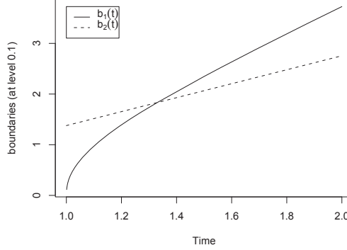
Figure 3: Boundaries for the Brownian bridge
