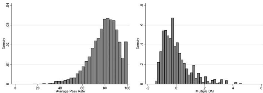
Figure 2: Average Pass Rates and MDM Score Density
