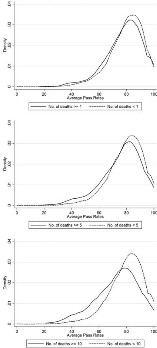
Figure 3: Average Pass Rates Density by Violence Intensity
