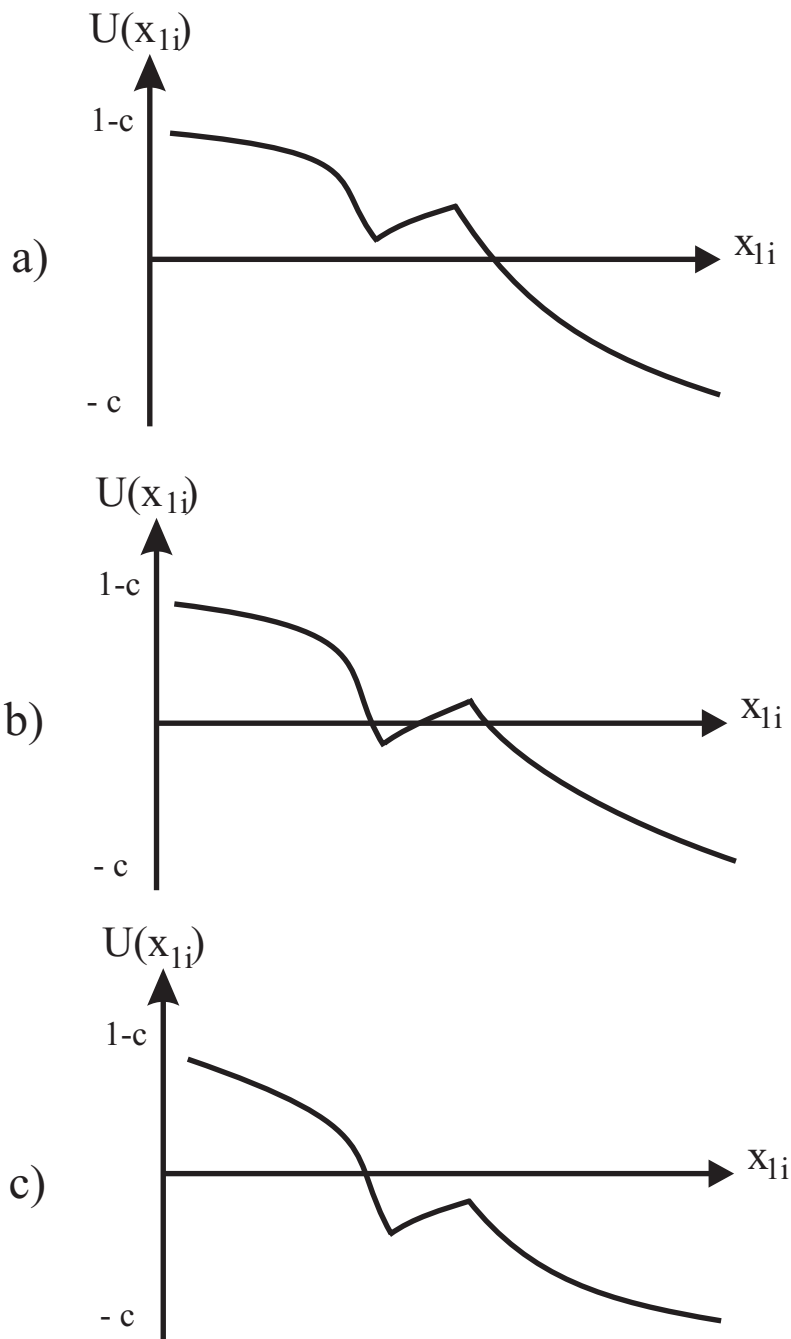
Figures: unique equilibrium in a) and c) at U(x_{1,i})=0 , multiple equilibria in b)
