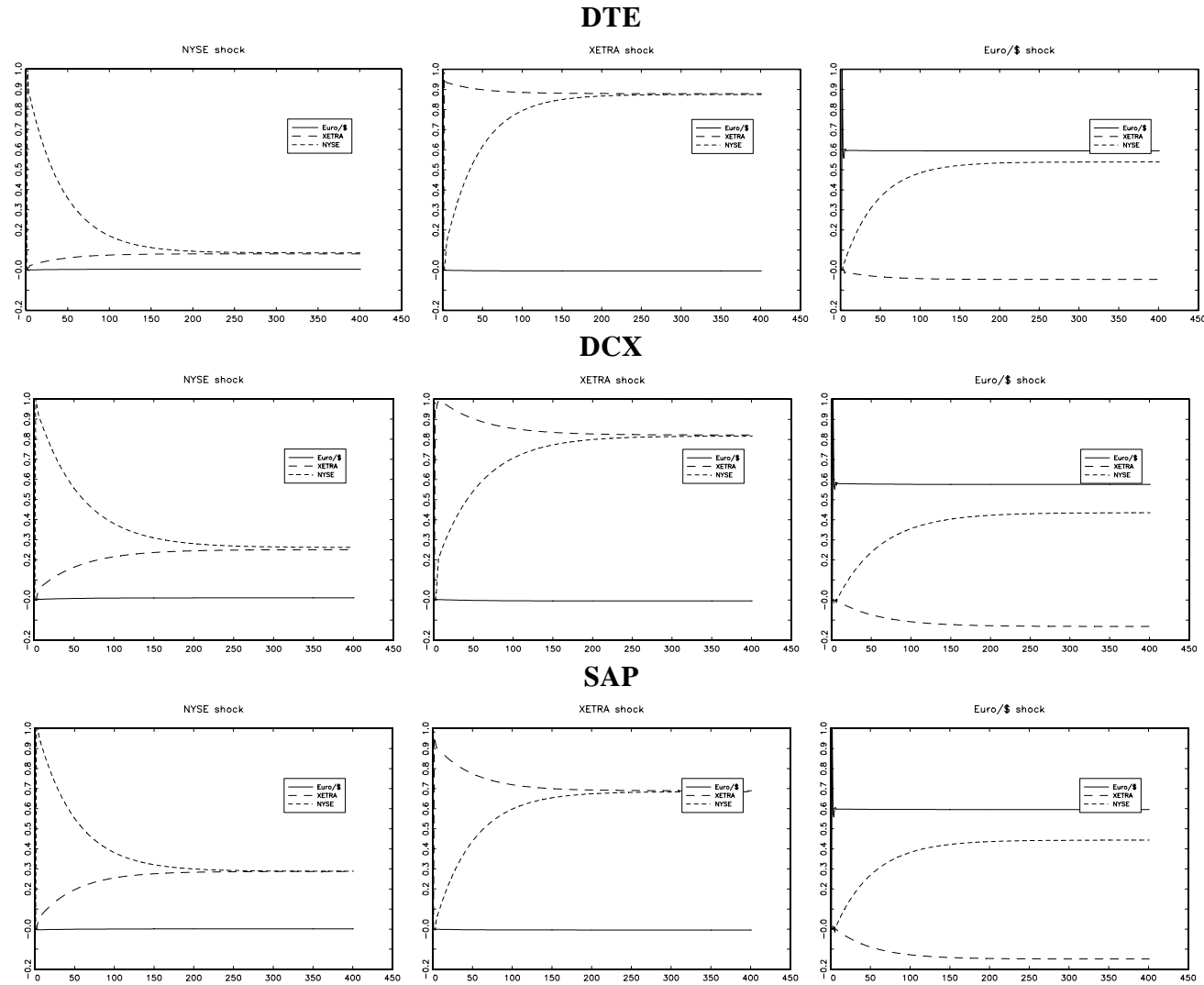
Figure 3 Impulse Response Functions
