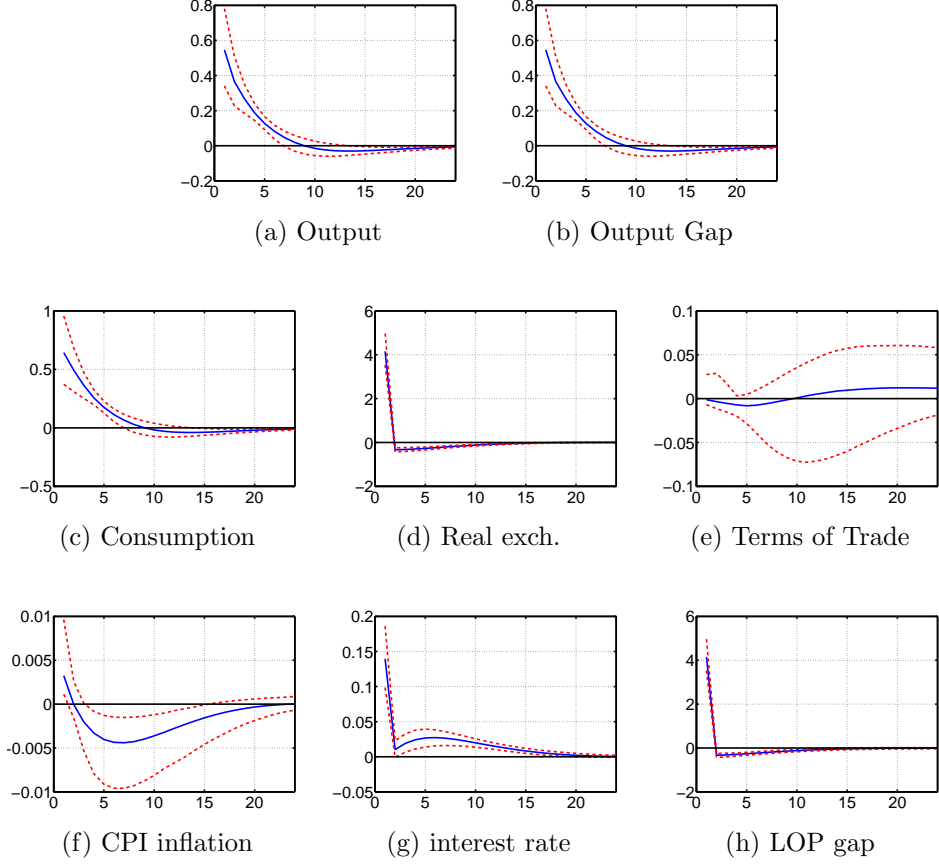
Figure 5: Impulse Responses (model IND) to a One Standard Deviation Shock to UIP condition with 95-Percent Confidence Interval
