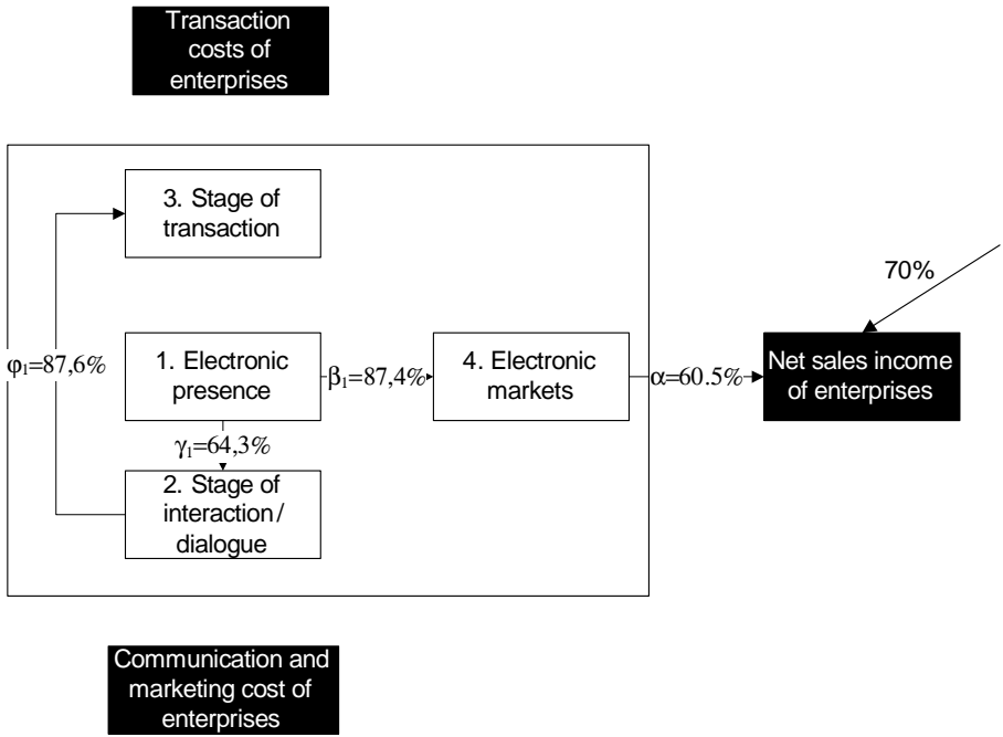
The final path model of the potential indicators
