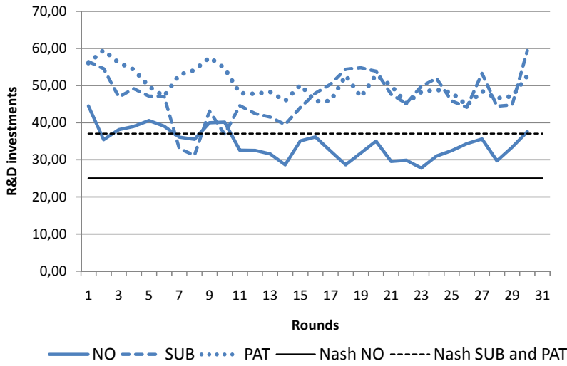
Figure 1: Observed and predicted R&D investments over rounds
