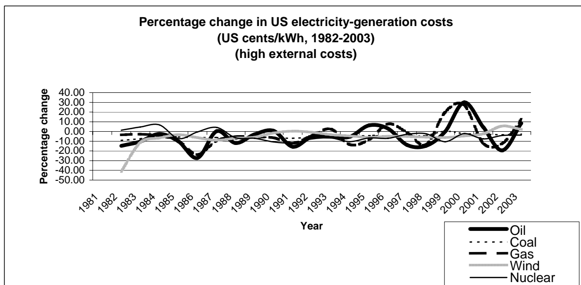
Figure 6 Percentage changes in U.S. electricity-generation costs (US cents/kWh) 1982-2003
