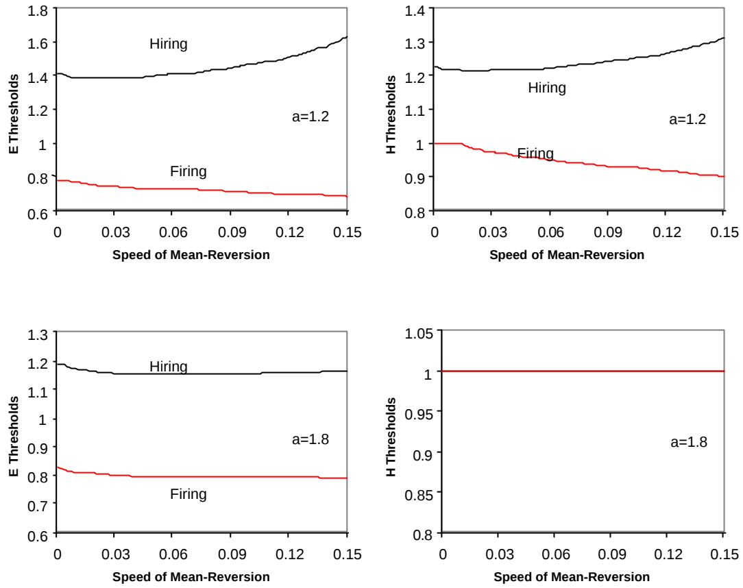
Figure 5: The Impact of \lambda Upon the Exchange Rates Thresholds and Hours Thresholds for \alpha = 1.2 and \alpha = 1.8
