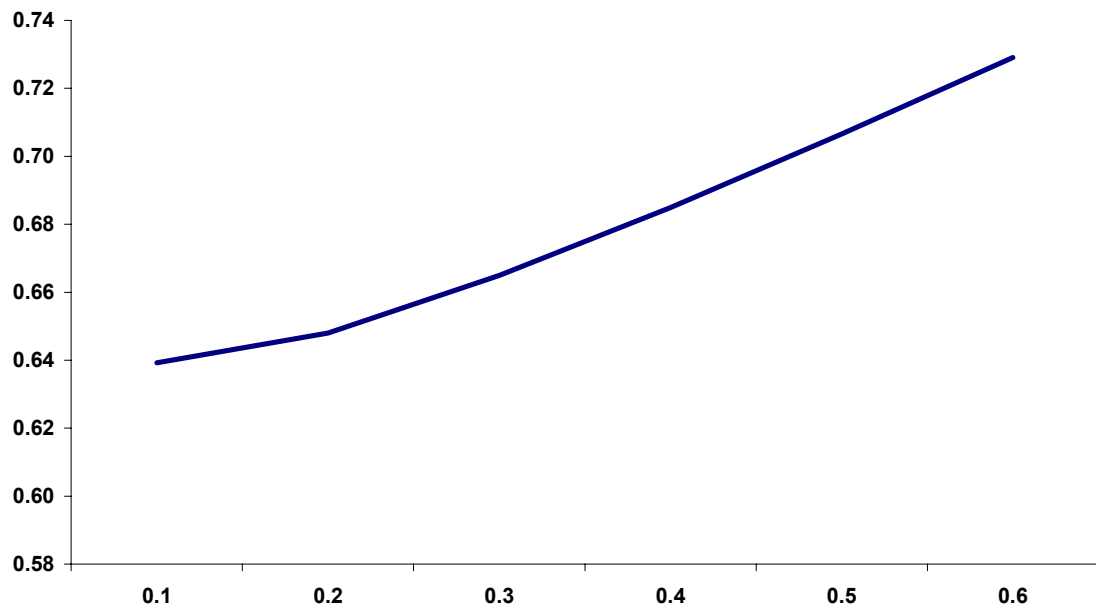
Graph of x^*(0.5, k)
