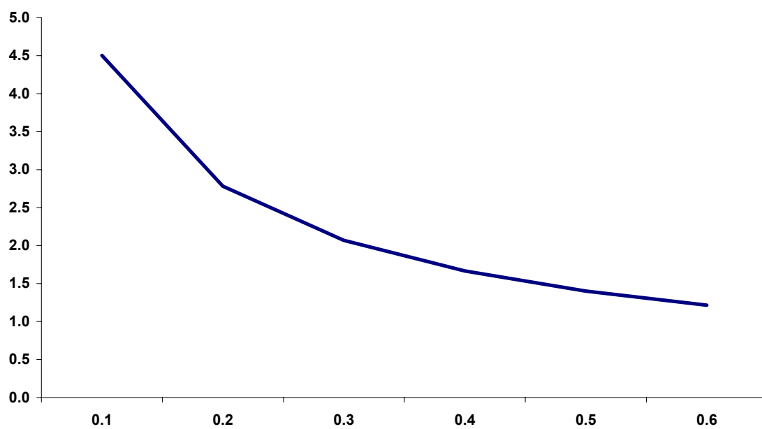
Graph of v^*(k)
