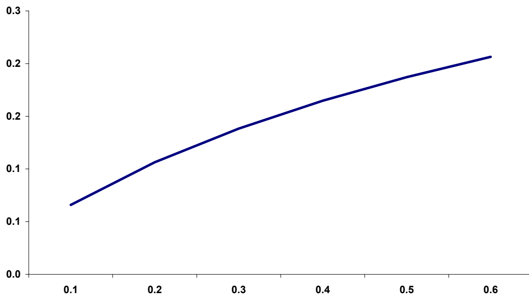
Graph of a(k)
