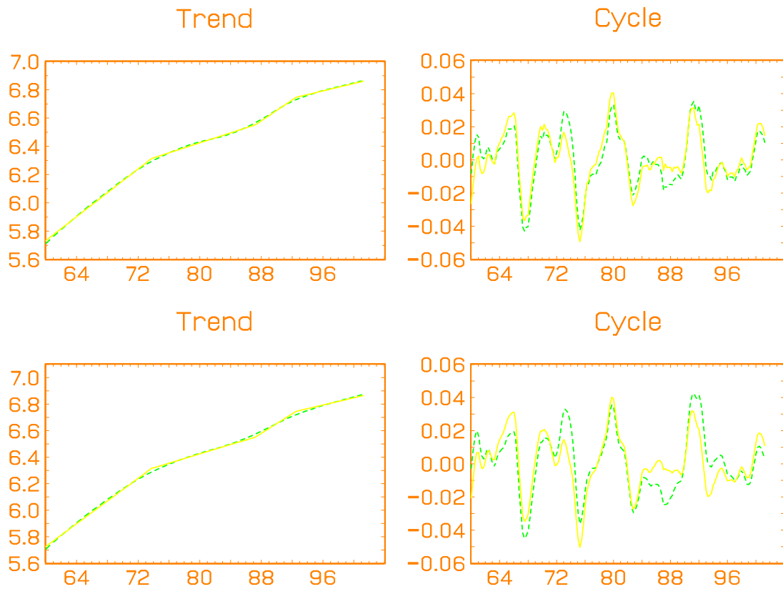
Figure 2: Trend and Cycle Components for Models I and III
