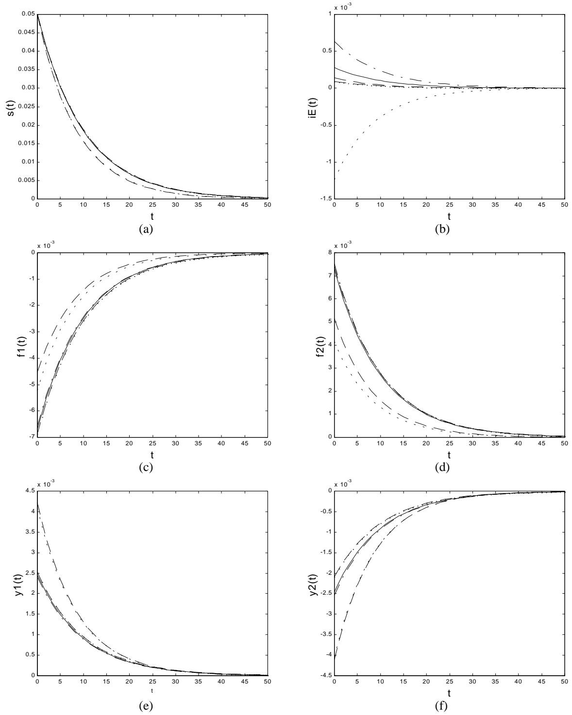
Figure 2a Asymmetric Case, \gamma_1 = 0.4 , \gamma_2 = 0.8 . Aggregate Objective Function ECB — Nash, --- Pareto, .... (1,2), - · - (1,3), - - - (2,3)
