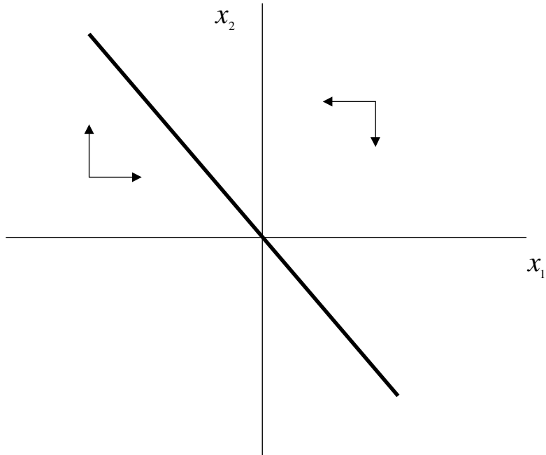
Figure 1: E-stable continuum when \pi_{11} + \pi_{22} < 1
