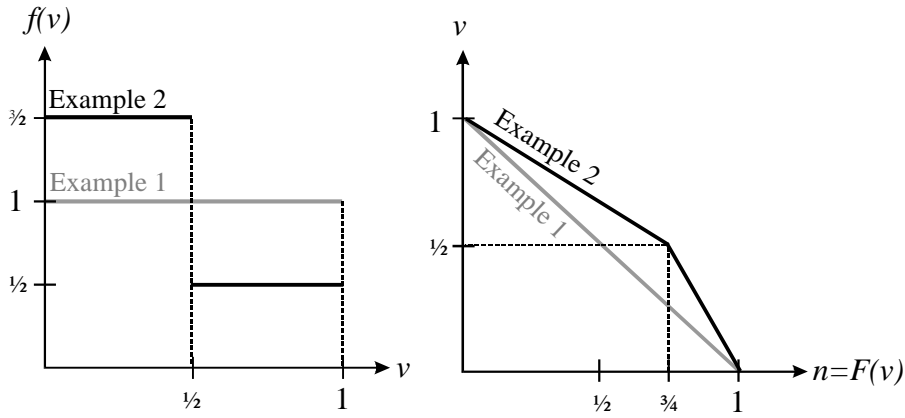
Figure 2. Linear and Kinked Demand for Entry
