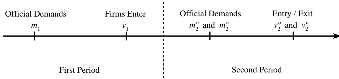
Figure 1. The Timing of the Repeated Extortion Game
