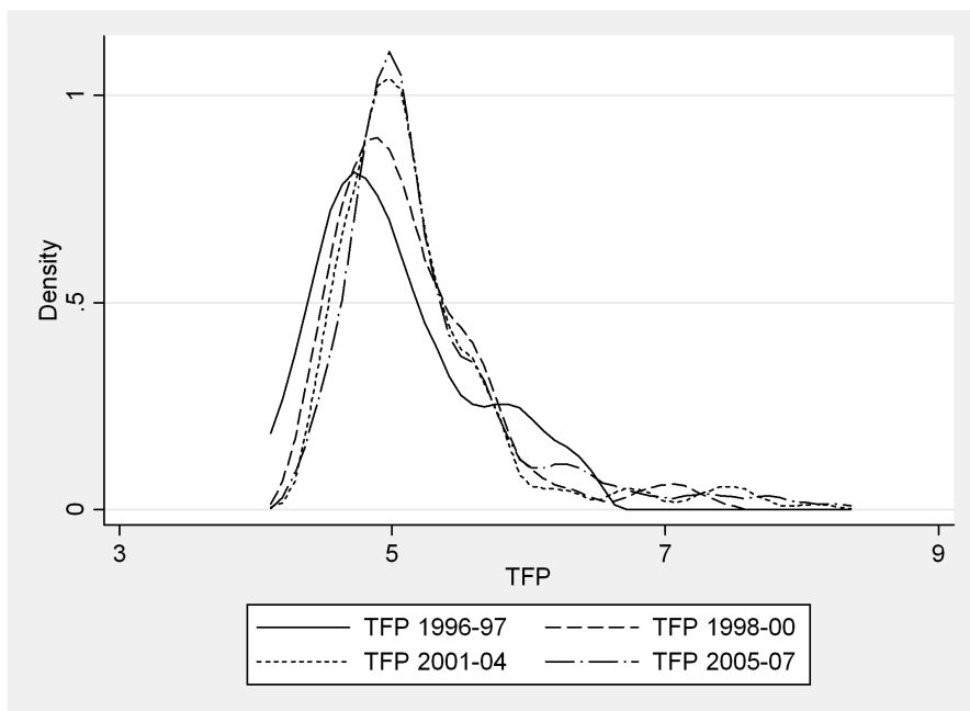
Figure 2: Productivity density function
