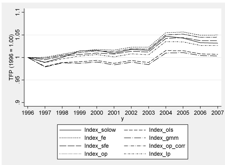
Figure 1: Weighted productivity index
