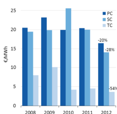
Figure 12. Control power prices as yearly averages. Products are aggregated to symmetric base, as in Figure 10. Relative changes compared to 2008.
