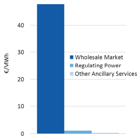
Figure 9. The costs of energy and ancillary service provision per MWh of consumed electricity. Control power is a very small market when compared to the wholesale market for energy (2011).
