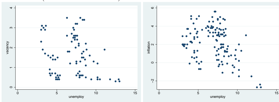
Figure 3: Scatter plots for vacancy ratios and unemployment rates (lhs) for eight EA as well as for inflation rates and unemployment rates (rhs) for eleven EA during the financial crisis (12 observations each)
