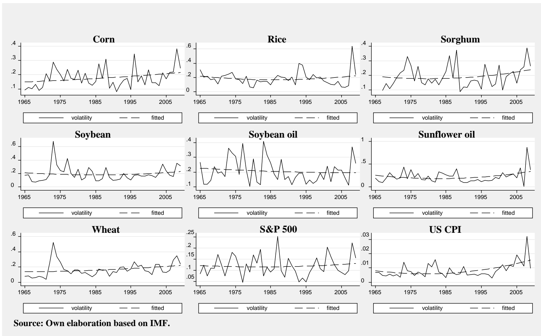
Graph 1: Historical volatility 1965–2009
