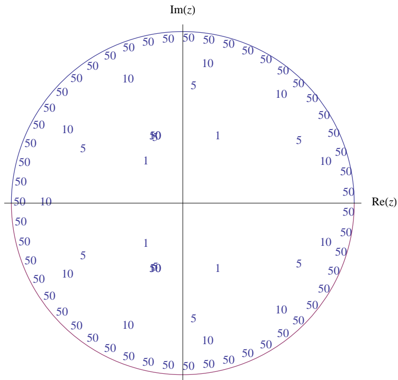
Figure 9: Zeroes of the characteristic polynomial h_{\ell,3}(x) for non-equal weights, in the complex plane. Each zero is indicated by the number “ \ell ”. The circle has centre 0 and radius 1.
