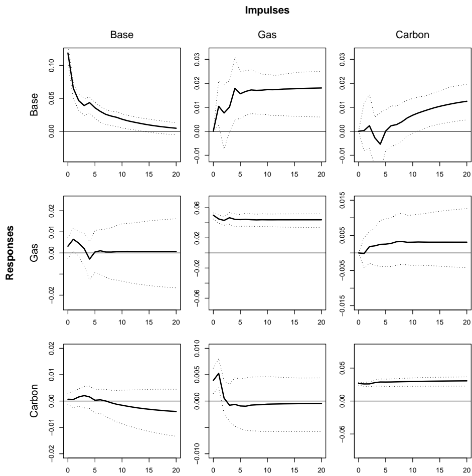
Figure 1: VECM orthogonal impulse responses
