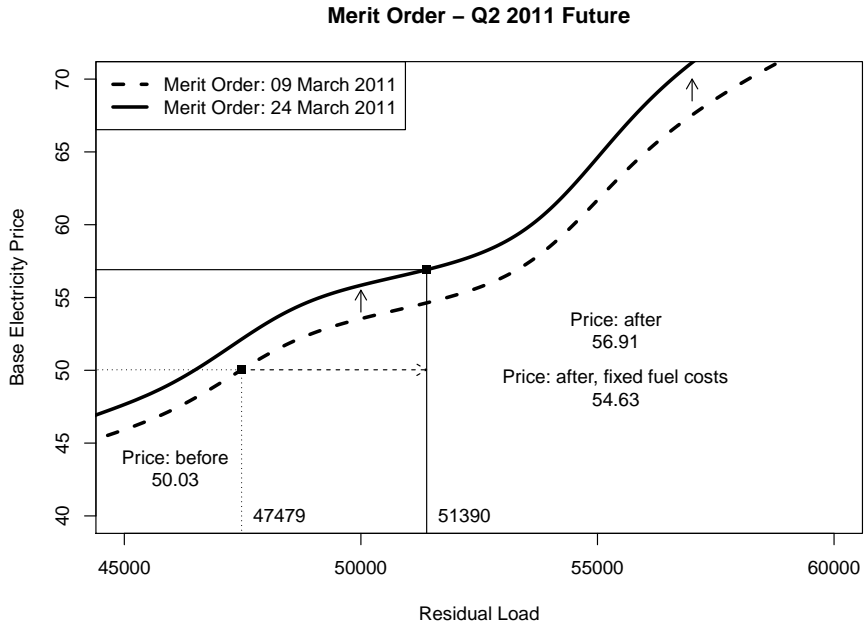
Figure 6: Shift of the merit order due to the moratorium
