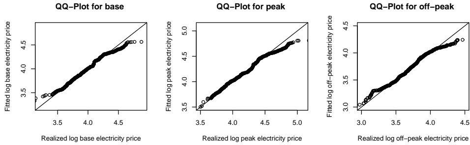
Figure 3: QQ-plot for the fit of the semiparametric model
