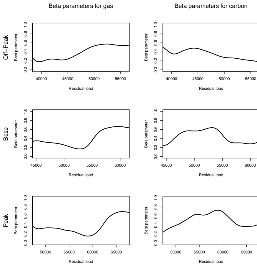
Figure 2: Semiparametric cointegration parameter estimates of fuel prices
