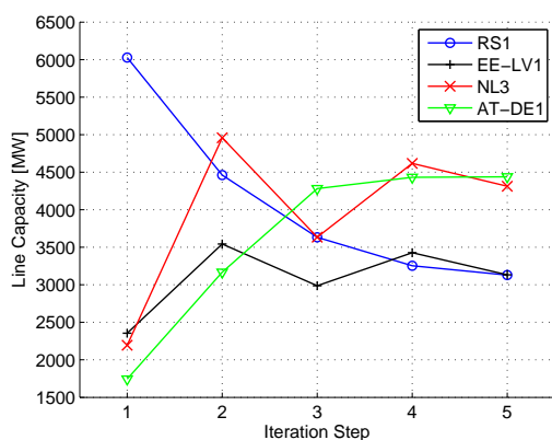
Figure 6: Development of optimal line capacities during the iteration in Scenario 1 (exemplary)
