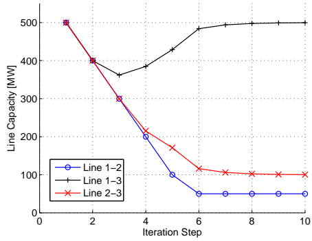
(a) Line capacities
