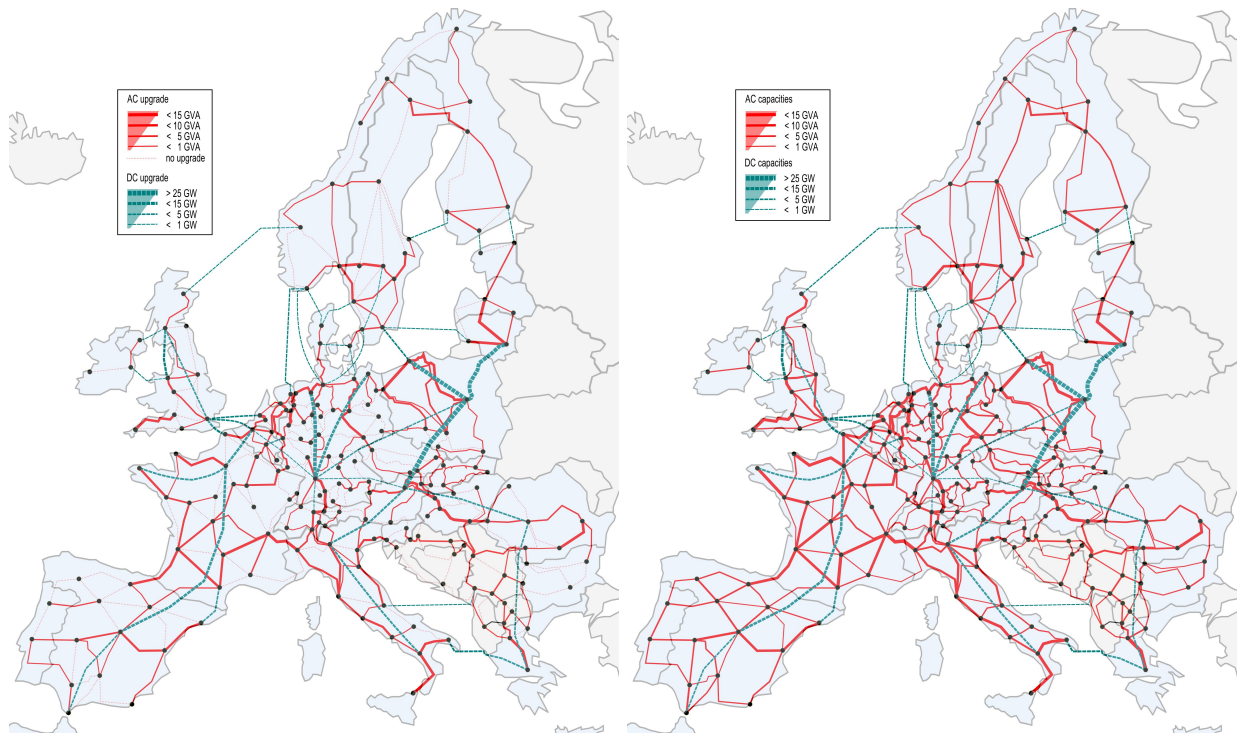
Figure 8: Grid upgrades between 2020 and 2050 (left hand side) and grid capacities in 2050 (right hand side) in Scenario 1
