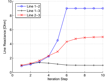
(b) Line reactances
