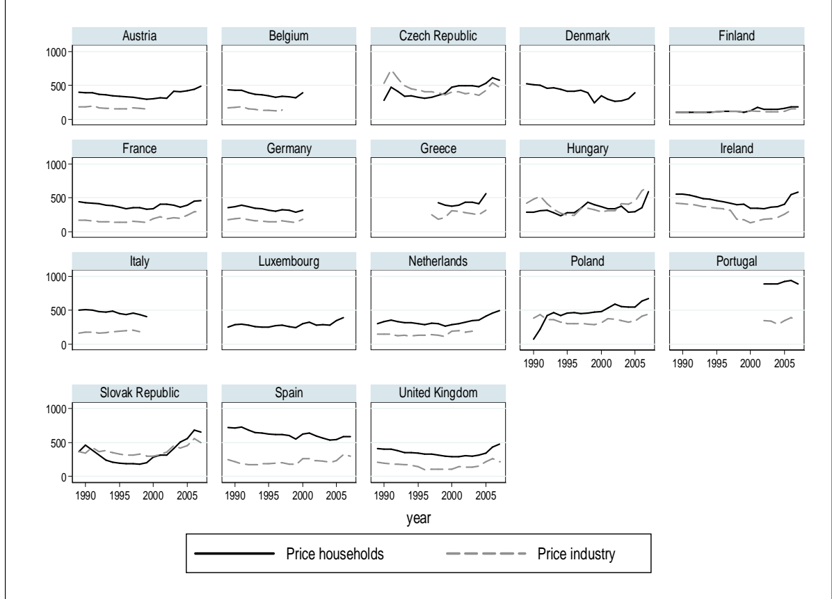
Figure 1: End-user prices [ \text{USD}_{2000}/10^7 \text{ kcal} ]
