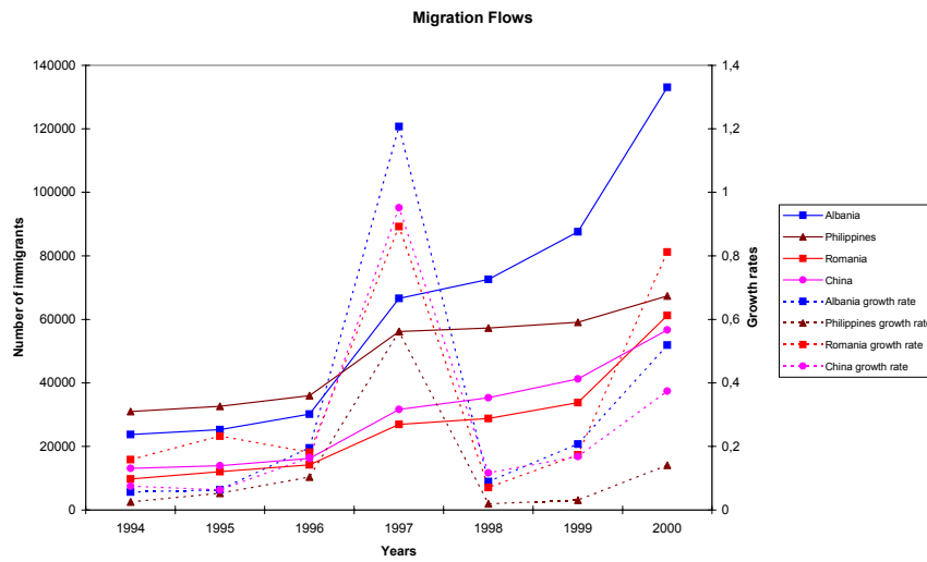
Figure 1: Migration jumps
