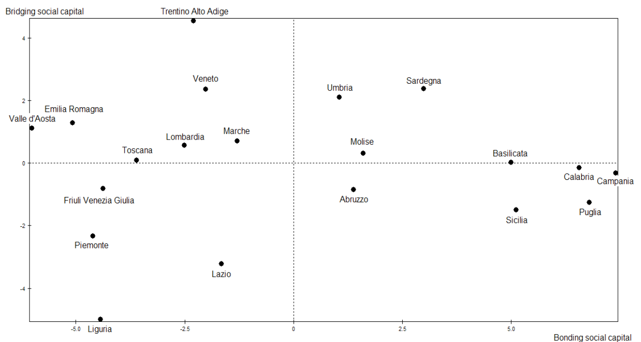
Figure 1. First factorial plan resulting from the PCA on informal networks
