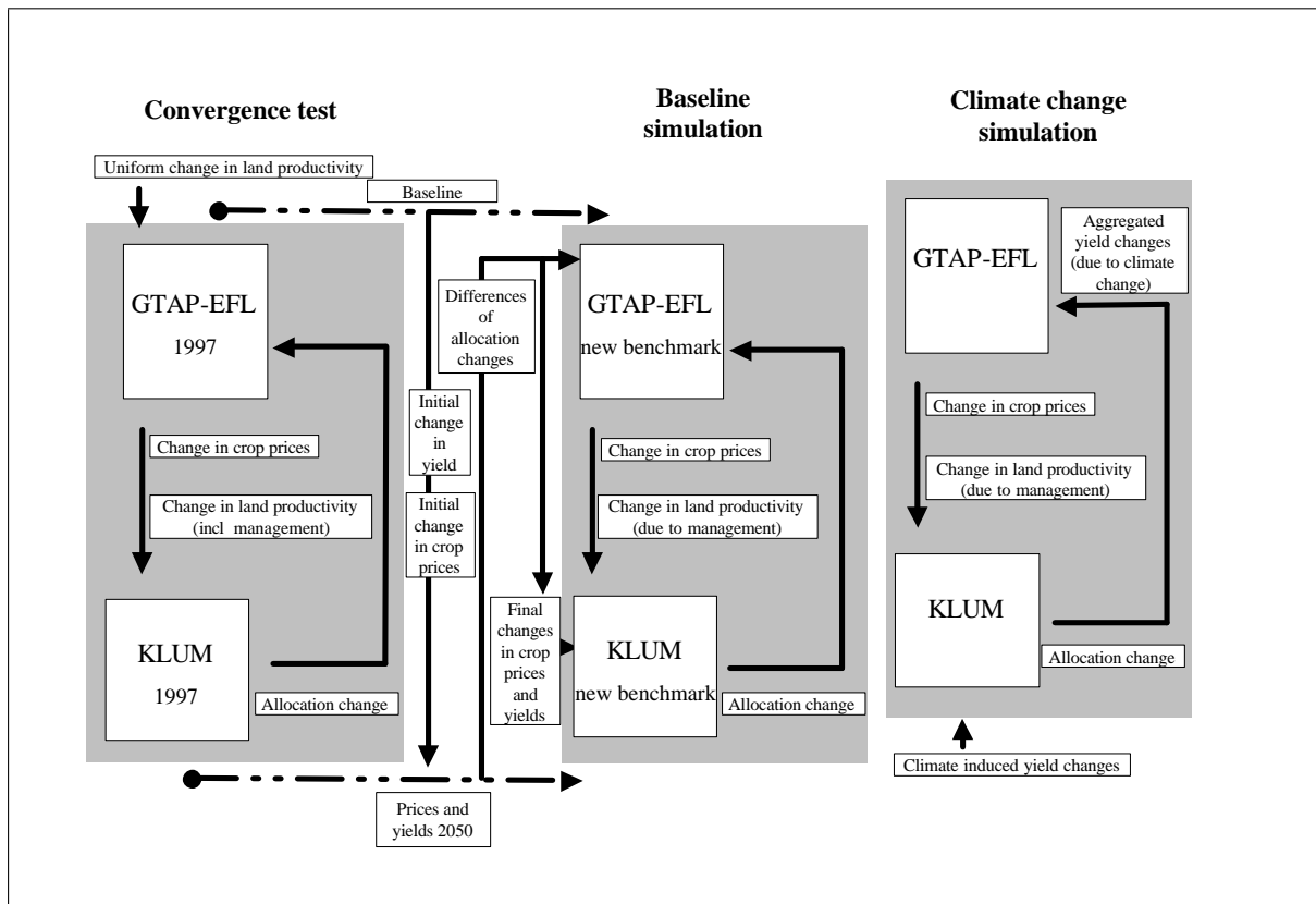
Figure 1. The coupling scheme of KLUM@GTAP: The coupling can be divided into 3 different procedures. For further details see the description in the text.
