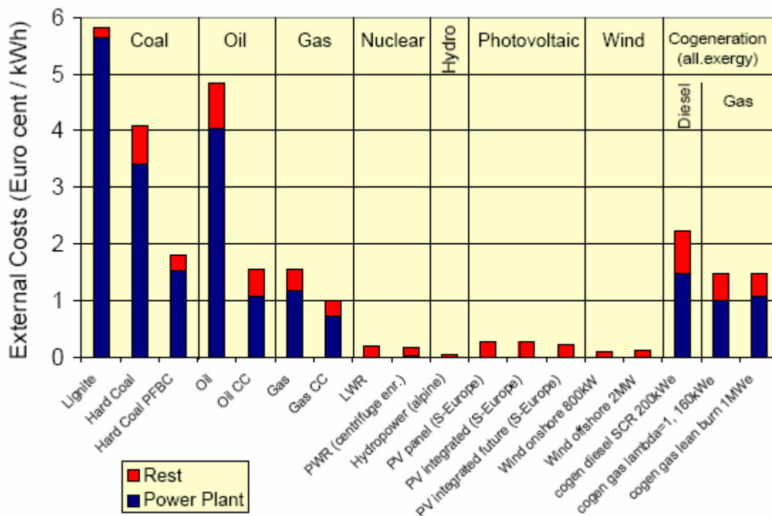
Figure 2. External costs of current and advanced electricity systems, associated with emissions from the operation of power plant and with the rest of energy chain. Source: ExternE-Pol, 2004.
