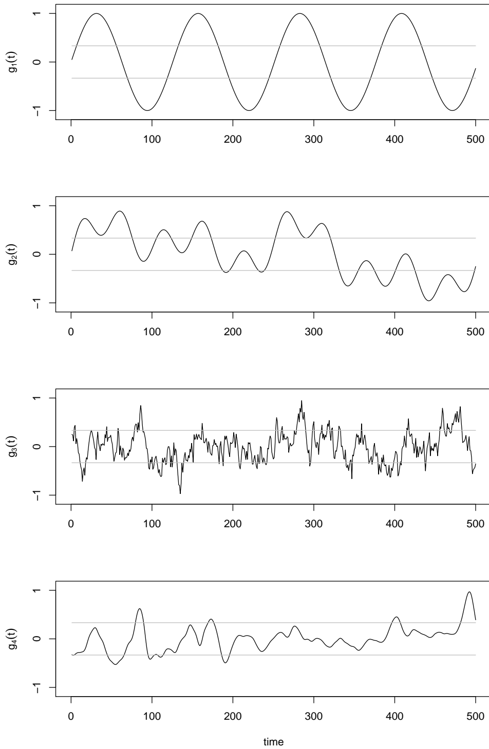
Figure 1: Different cycle functions with the appropriate thresholds \tau^s (grey lines).
