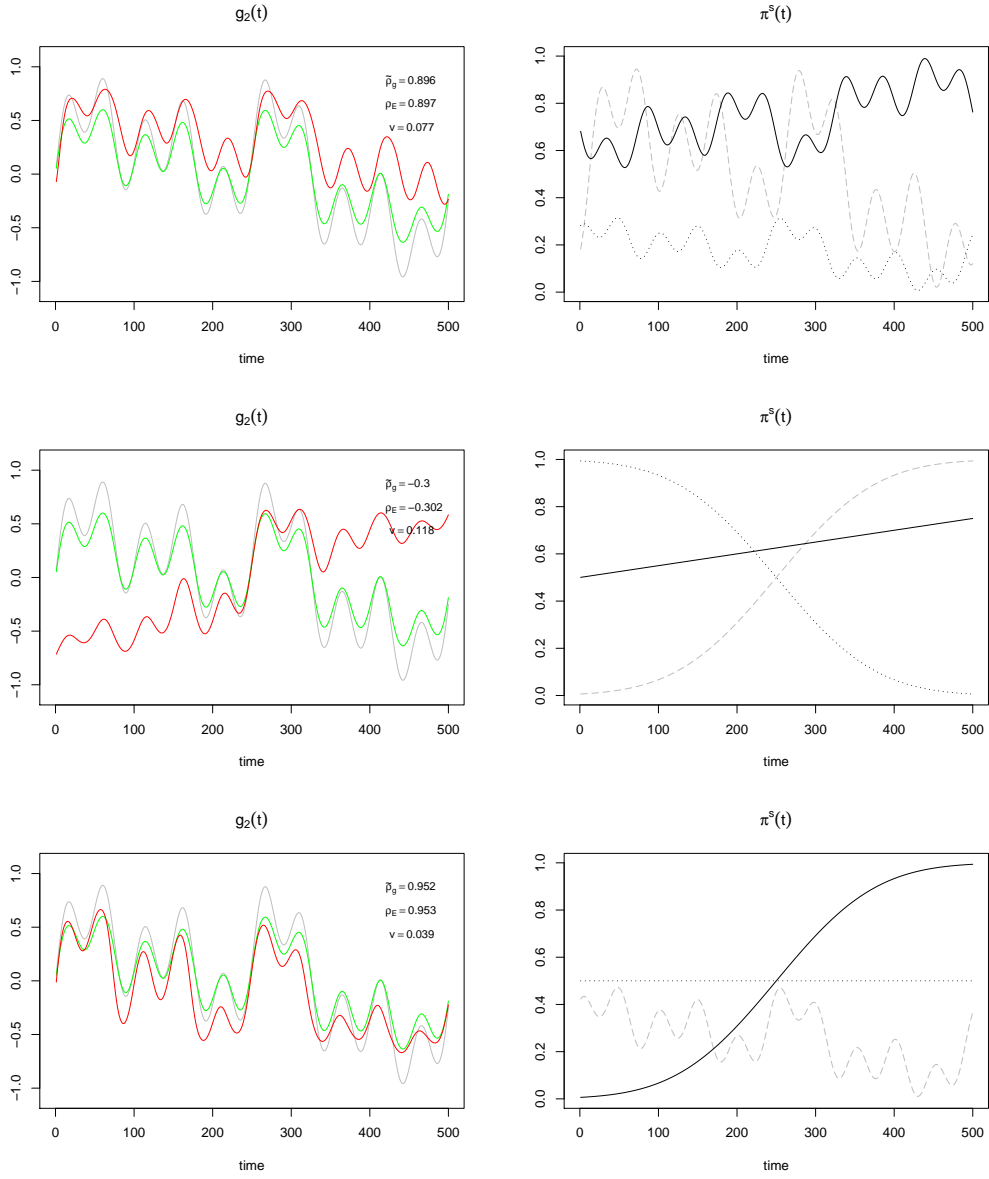
Figure 5: Effects of bias patterns II. Left: cycle function g_2(t) (—), unbiased mean function E_t(y) (—) and biased mean function E_t(y^{obs}) (—). Right: acceptance rates \pi^+(t) (- - -), \pi^-(t) (—) and \pi^s(t) (· · ·). From top to bottom: Cycle-shifted (with \pi^+(t) = \pi_{2,1}^S(t - 12) , \pi^-(t) = 1 - \pi_{2,2}^S(t + 3) and \pi^s(t) = \pi_{2,3}^S(t + 12) ), monotone (with \pi^+(t) = \pi_{100}^M(t) , \pi^-(t) = \pi_{2000}^L(t) and \pi^s(t) = 1 - \pi_{100}^M(t) ) and mixed (with \pi^+(t) = \pi_{2,2}^S(t + 12) , \pi^-(t) = \pi_{100}^M(t) and \pi^s(t) = 0.5 ) patterns.
