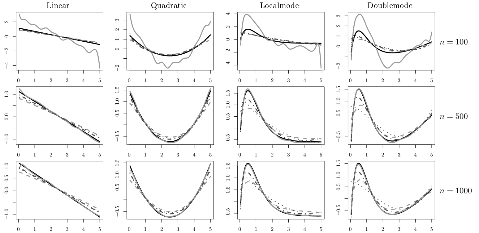
Figure 6: Survival additive model: True functions (black solid lines) and average estimated functions (grey solid lines P -splines based on AIC, grey dashed lines P -splines based on REML, black dots FP_2 and black dashed lines FP_4 estimates).
