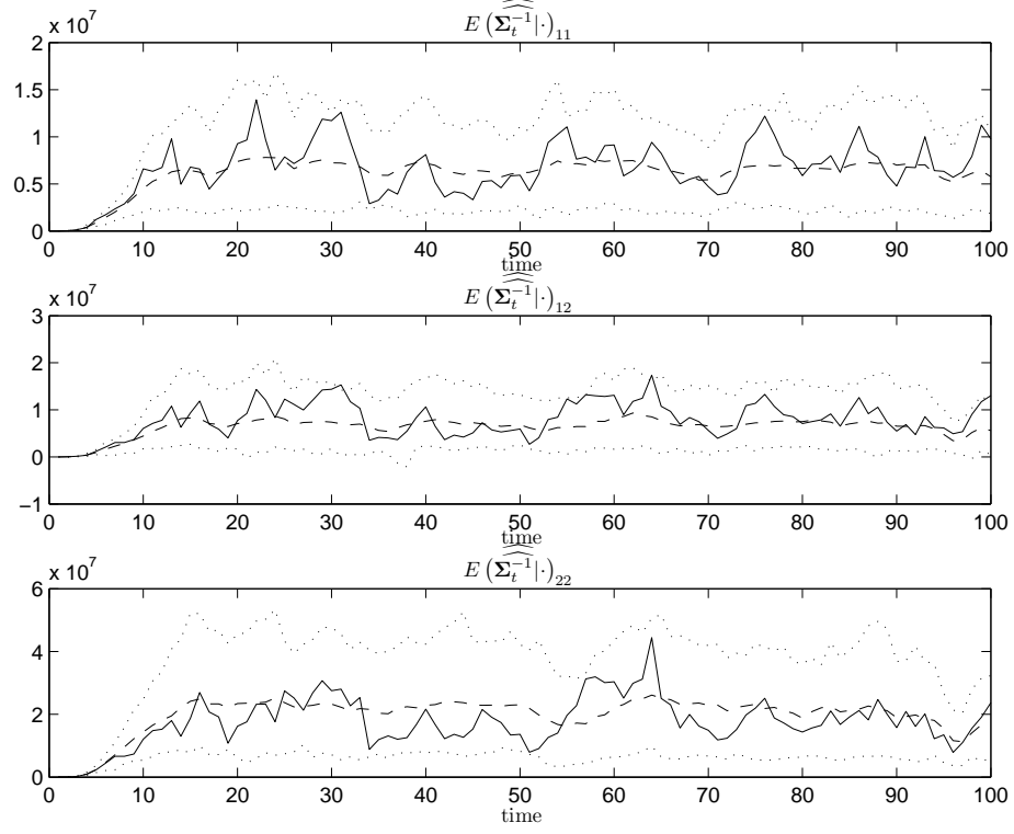
Figure 3: Plot of the elements of E(\widehat{\widehat{\Sigma_t^{-1}}|\cdot}) for the example data set, where the dotted line is the 95% hpdi, the solid line denotes the true values, and the dashed line corresponds to the mean of the sampling observations.
