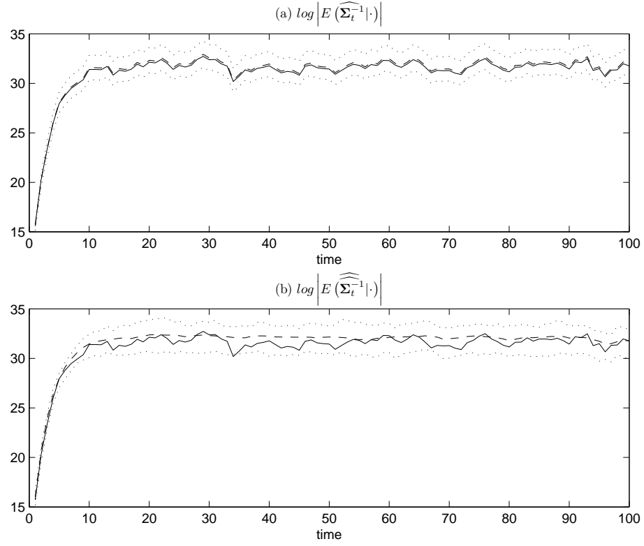
Figure 2: Plot of the estimates of \log |E(\widehat{\Sigma_t^{-1}}|\cdot)| (---), \log |E(\widehat{\widehat{\Sigma_t^{-1}}}|\cdot)| (- - -), their 95% hpdi ( \cdots ), and their true values (—) for the example data set.
