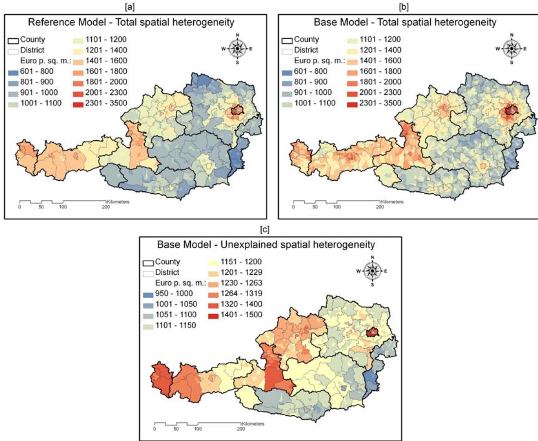
Figure 4: Distribution of spatial heterogeneity (evaluated at the average effect). [a] Total spatial heterogeneity in the reference model. [b] Total spatial heterogeneity in the base model (including neighborhood covariate effects). [c] Remaining unexplained spatial heterogeneity in the base model (scale differs from above).
