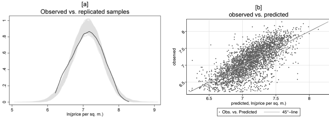
Figure 7: [a] kernel densities for the distribution of observed house prices (black line) vs. simulated prices according to the base model (grey line), [b] scatter plot of observed vs. predicted log house prices per sq. m.
