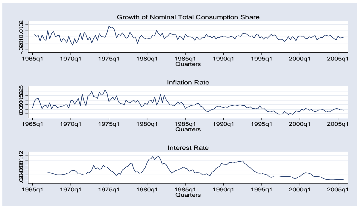
Figure 5: Additional Variables
