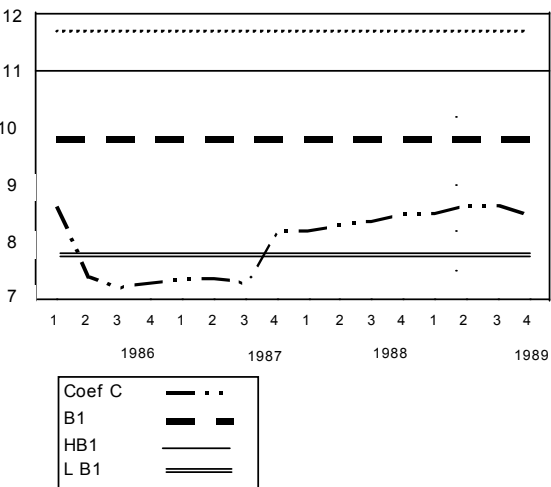
Figura 11 CONSTANT
