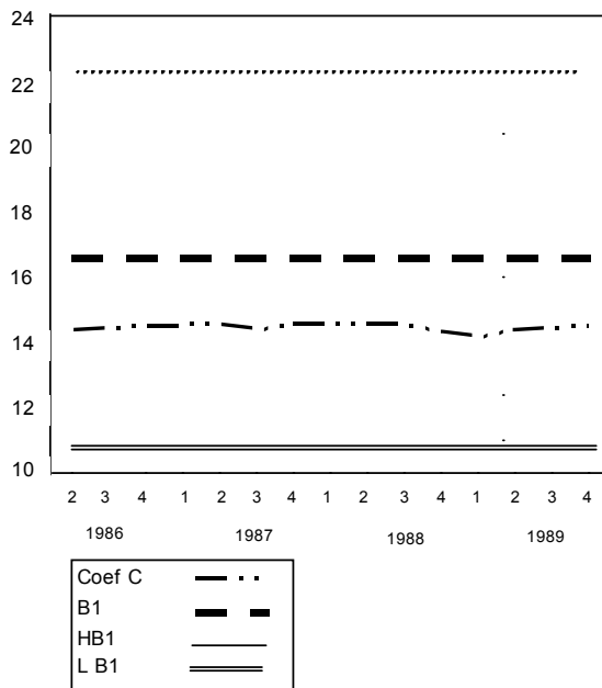
Figura 10 DIFTCINF
