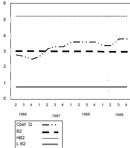
Figura 11 CONSTANT
