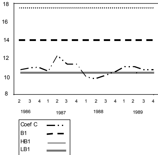
Figura 18 CONSTANT
