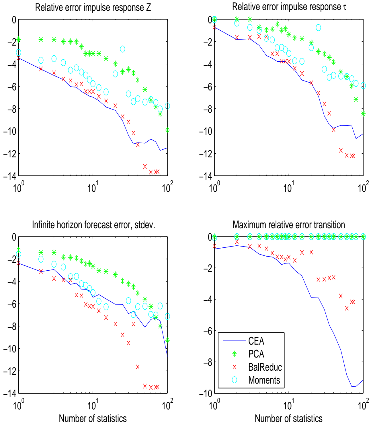
Figure 2: log10 of approximation errors in K , stochastic growth model with model reduction, n_P = 1
