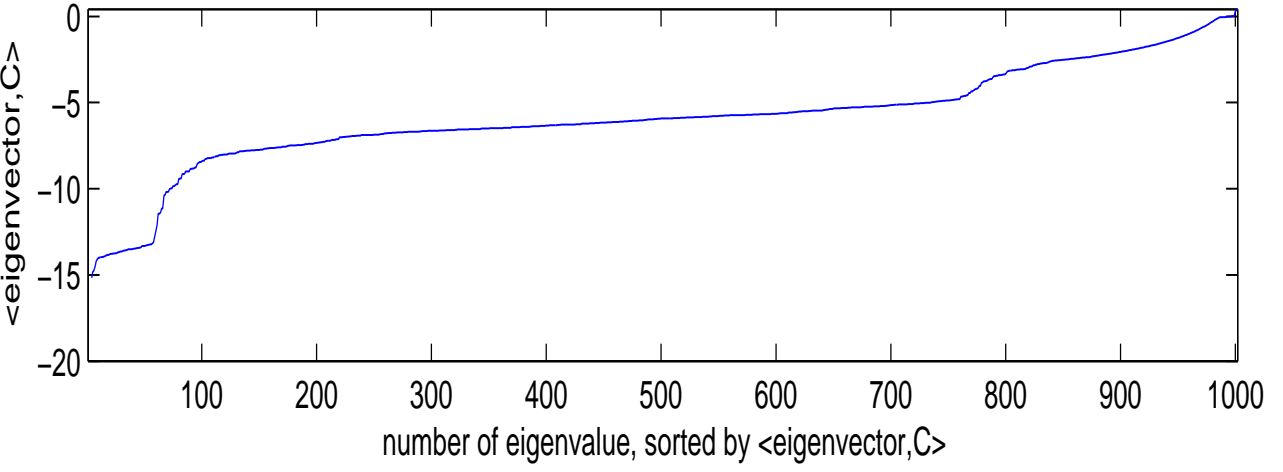
Figure 6: Popov-Belevitch-Hautus test for exact aggregation, growth model, n_P = 1
