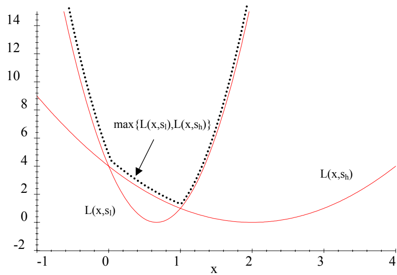
Figure 1: Loss functions
