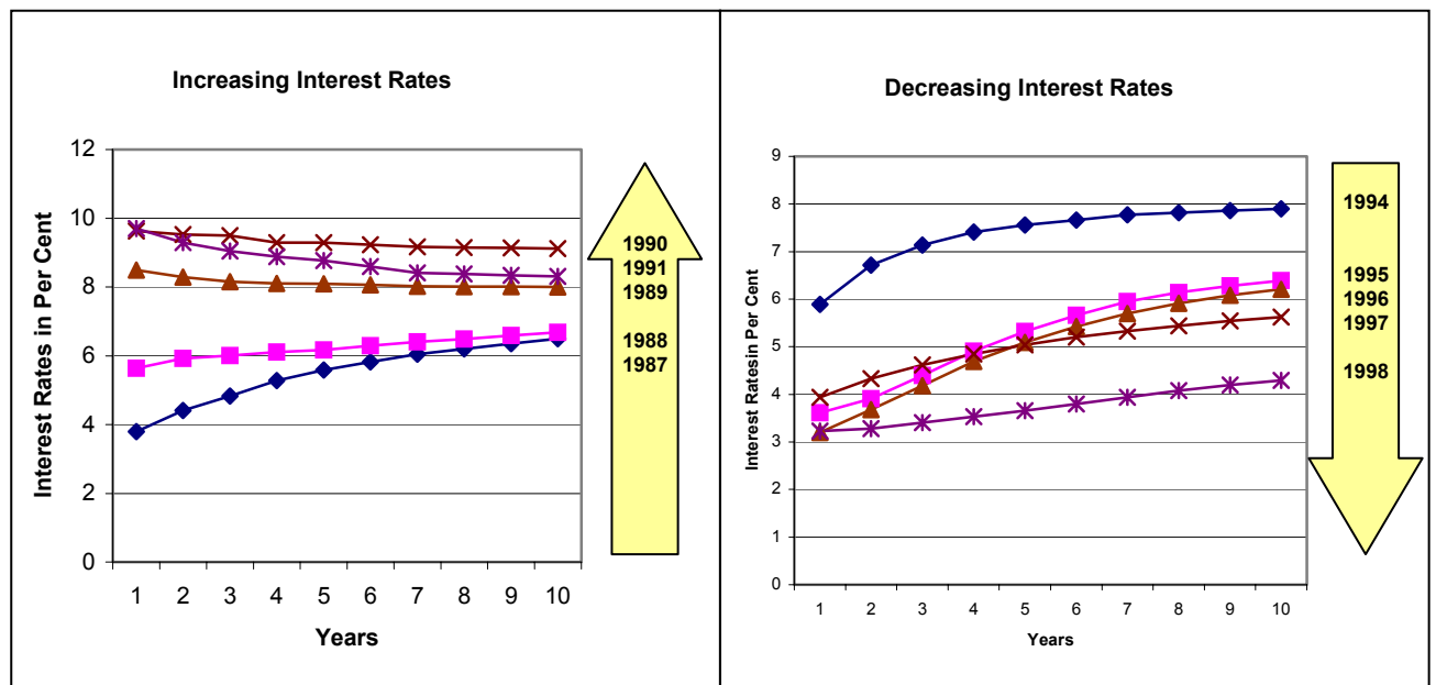
Figure 2: Scenarios of Rising and Falling Interest Rates
