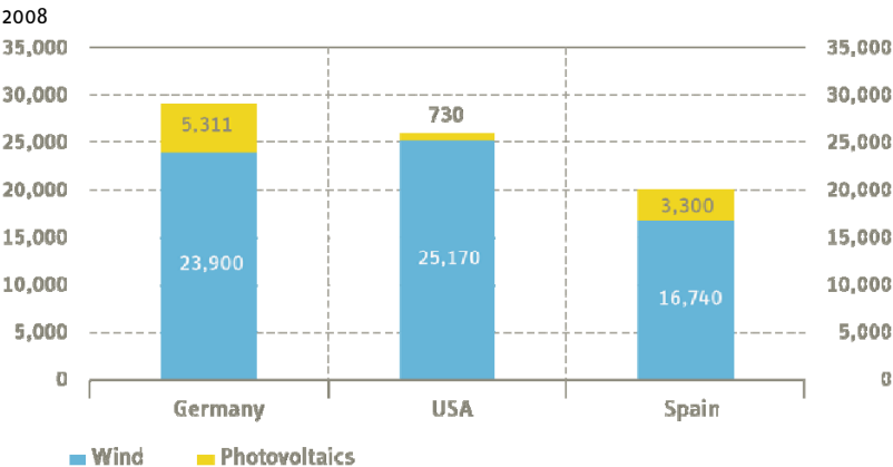
Figure 3: Installed Capacities of Wind Power and PV (REN21)
