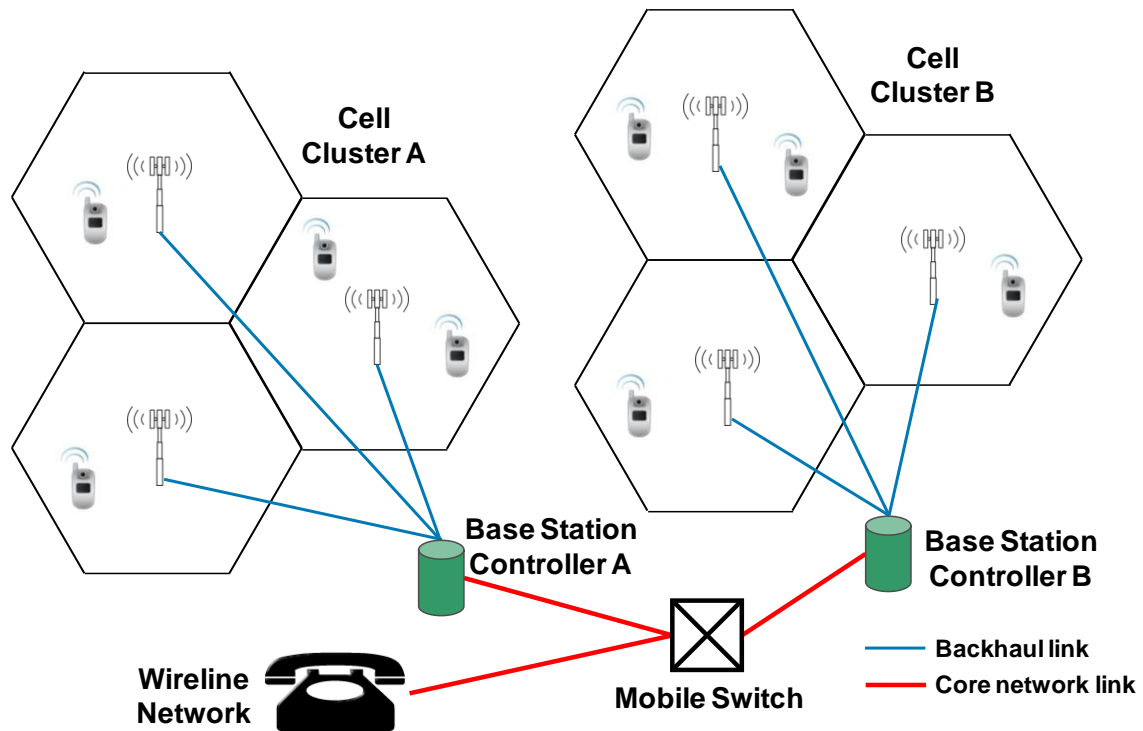
EXHIBIT 1: Mobile Network Schematic
