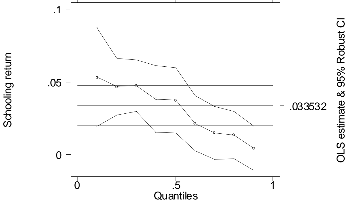
Quantile regression coefficients 95% CI's, Bootstrap estimates reps=1000
