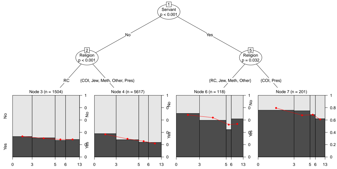
Figure 7: Q-Q Logistic regression tree for Belfast. The plots in the leaves give spinograms for school attendance versus sibling size.
