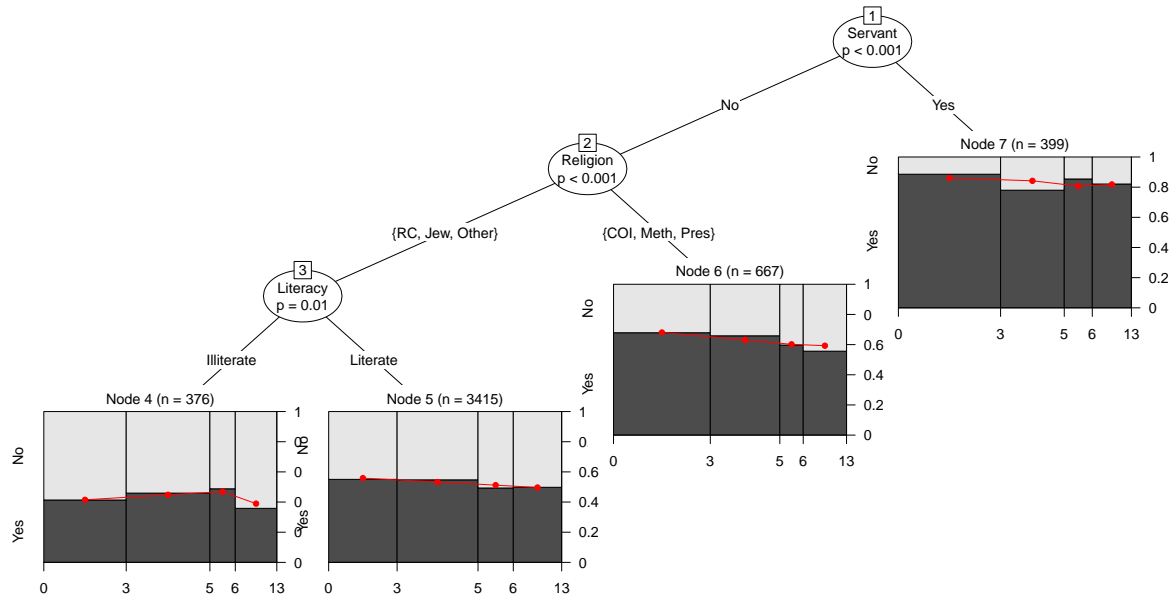
Figure 8: Q-Q Logistic regression tree for Dublin. The plots in the leaves give spinograms for school attendance versus sibling size.
