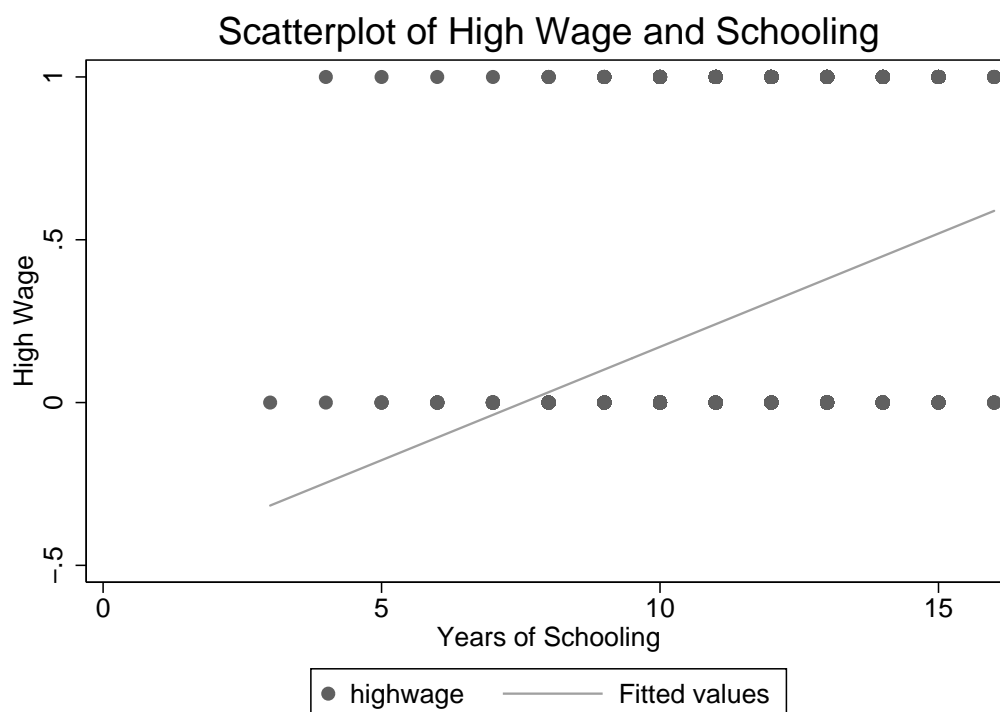
Figure 4: A Problem With OLS
